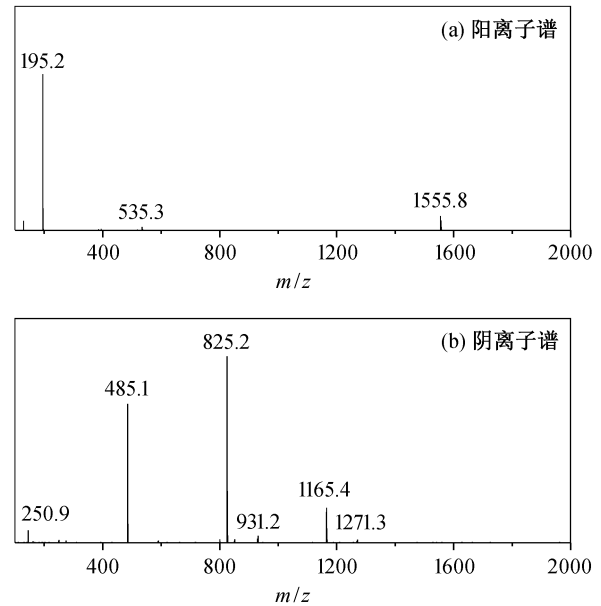
图4 [C_8mim][PF_6] 萃取0.1 mol/L ReO_4^- 后离子液体相的ESI-MS谱
